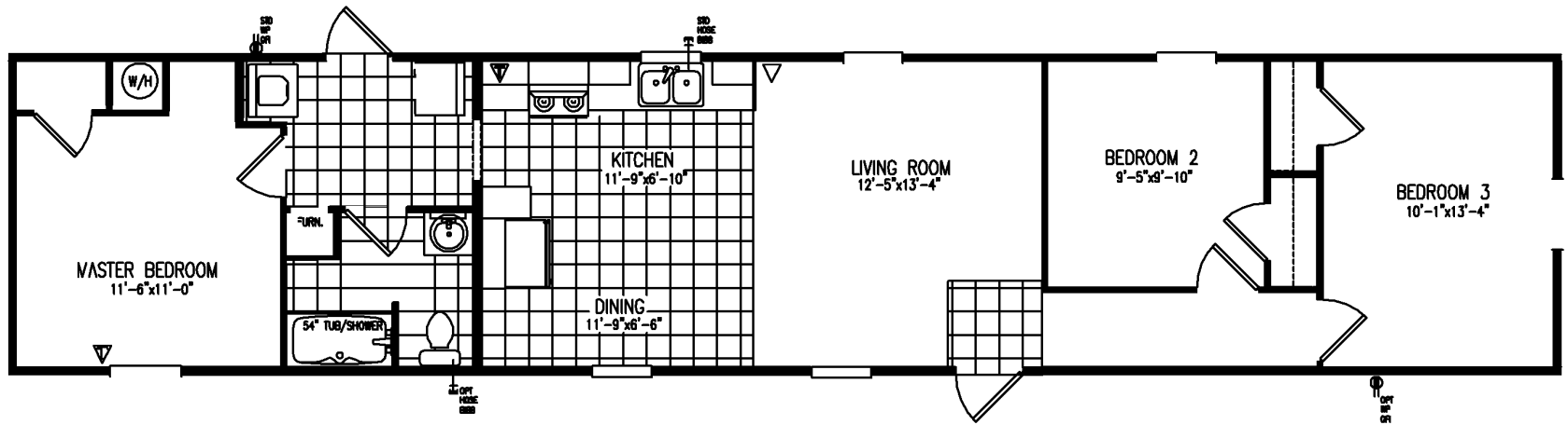
MODEL A703-19-96 3 BR. ~ 1 BA. 14'-0 X 70'-0 ~ 902 SQ. FT.
